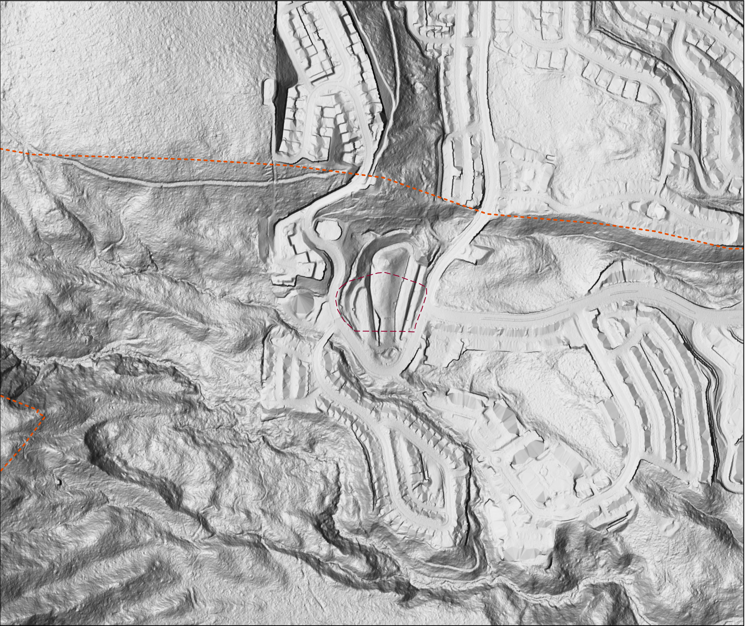
Figure 4: 2021 Lidar Hillshade
