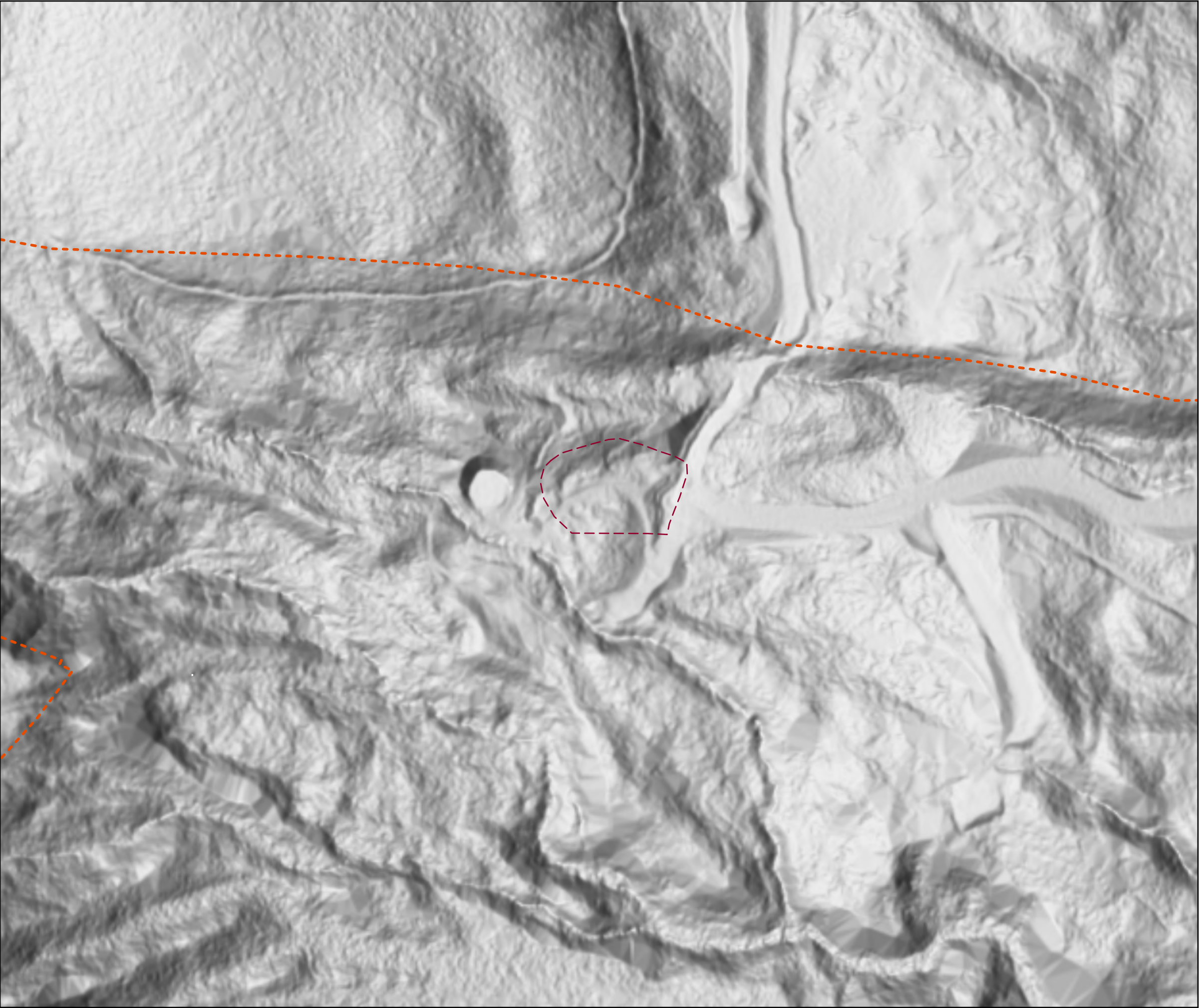
Figure 2: 2005 Lidar Hillshade
