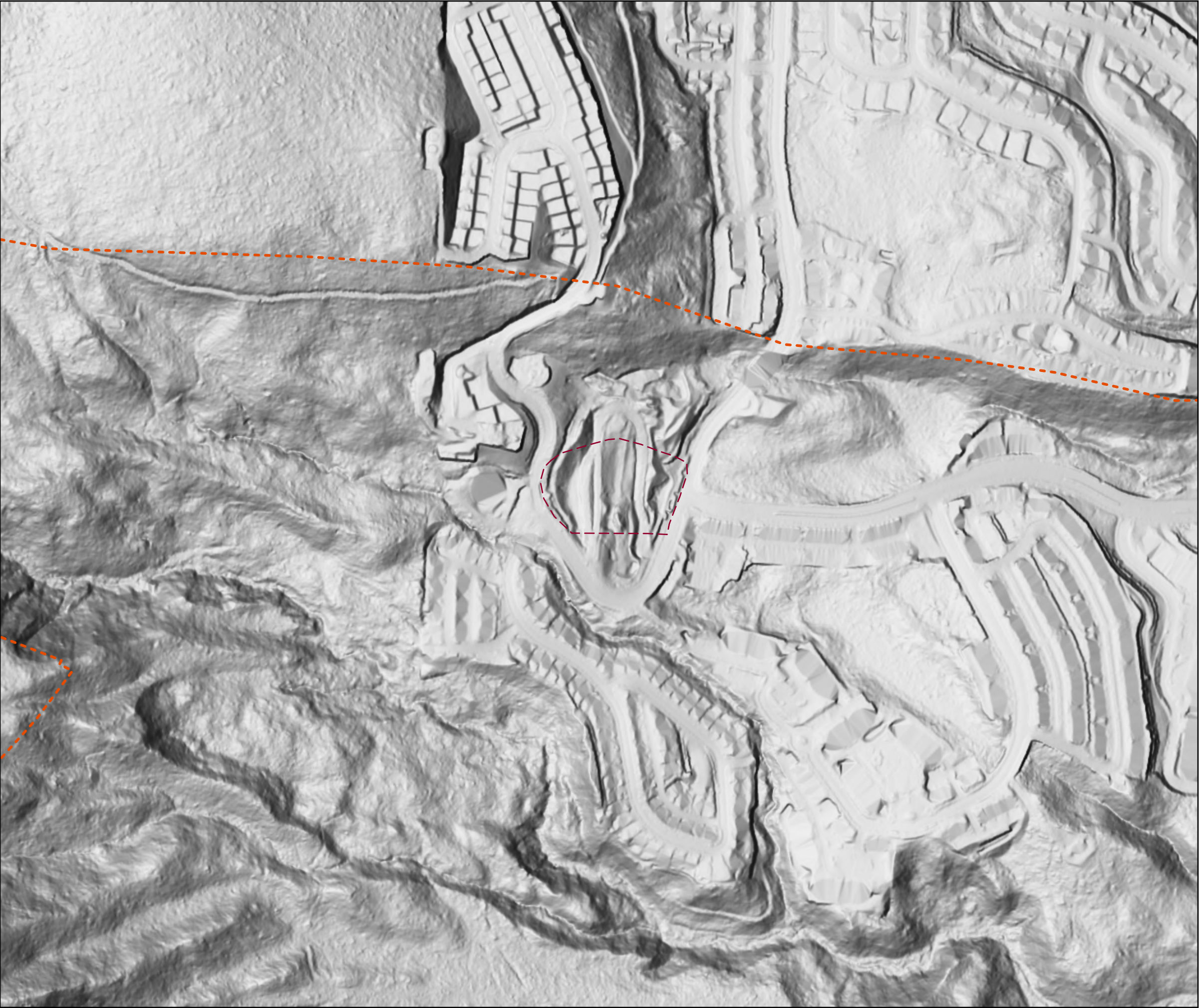
Figure 3: 2016 Lidar Hillshade
