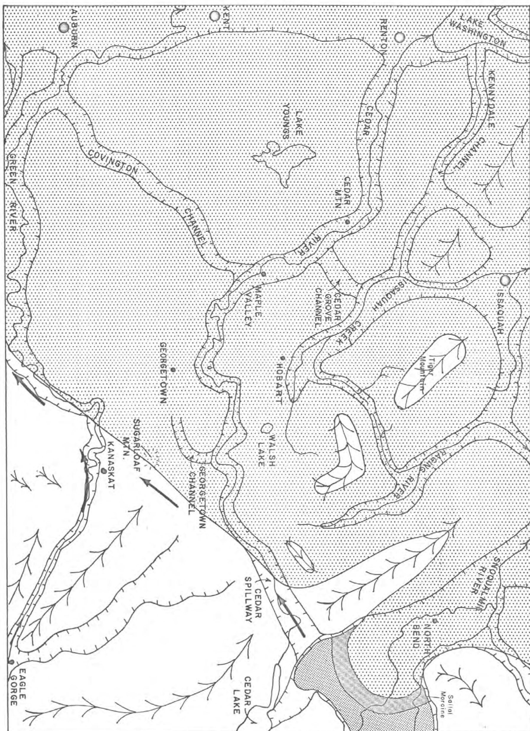
PHYSIOGRAPHIC MAP SHOWING ICE FRONT, GLACIAL LAKES, MORaine, AND DRAINAGE
