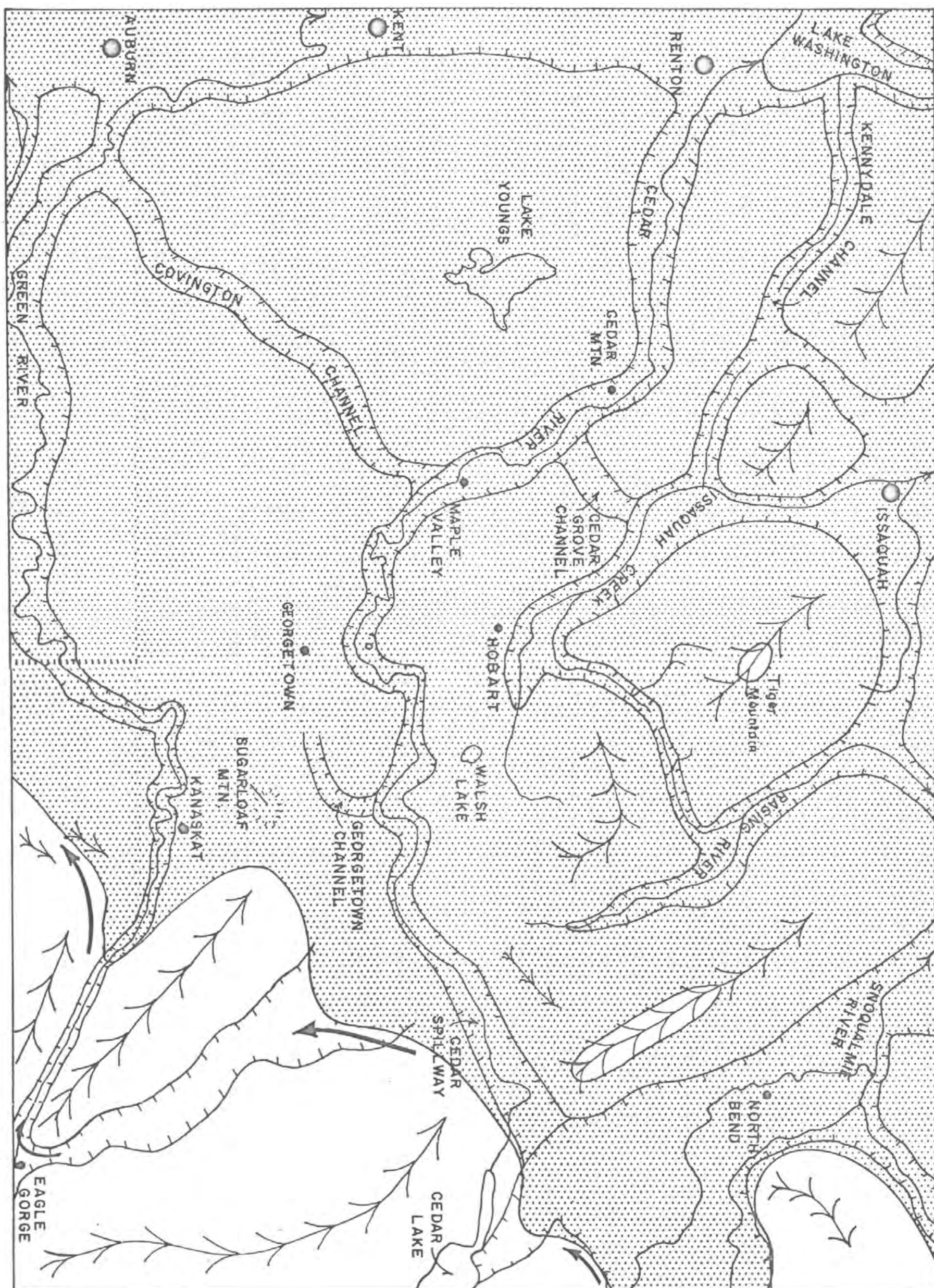
PHYSIOGRAPHIC MAP SHOWING ICE FRONT, GLACIAL LAKES, DELTAS, AND DRAINAGE
